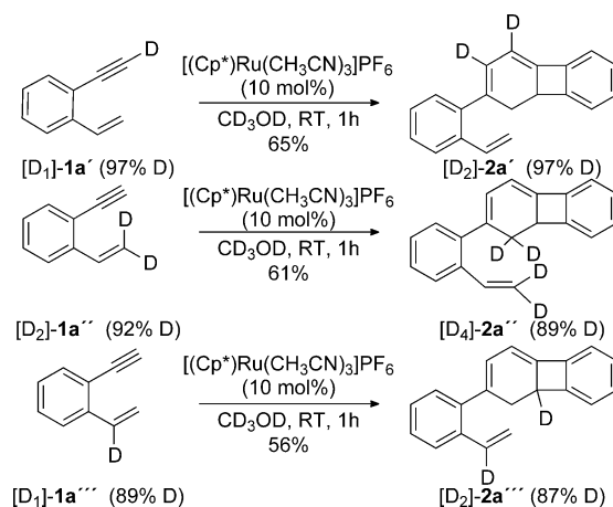
Scheme 2. Deuterium-labeling experiments.
